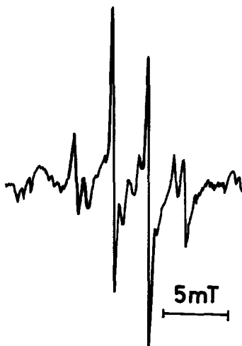
Fig. 1. E.s.r. spectrum of \cdot\text{C}_2\text{H}_5 radical obtained on photo-oxidation of 1,1-dimethylpropan-1-ol by Ce(IV) ammonium nitrate at 77 K [2].
